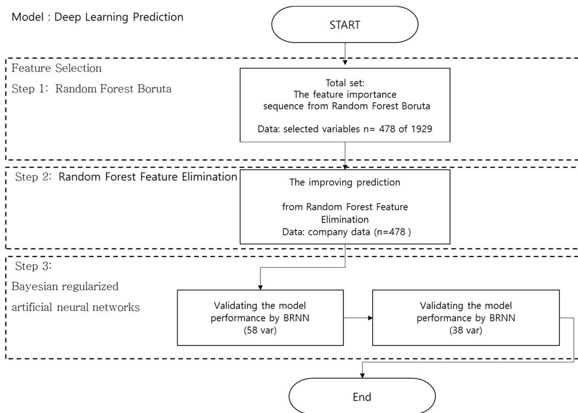
Figure 1. Analytic Algorithm Methodology: Deep Learning Prediction and Regression Prediction Algorithms.
