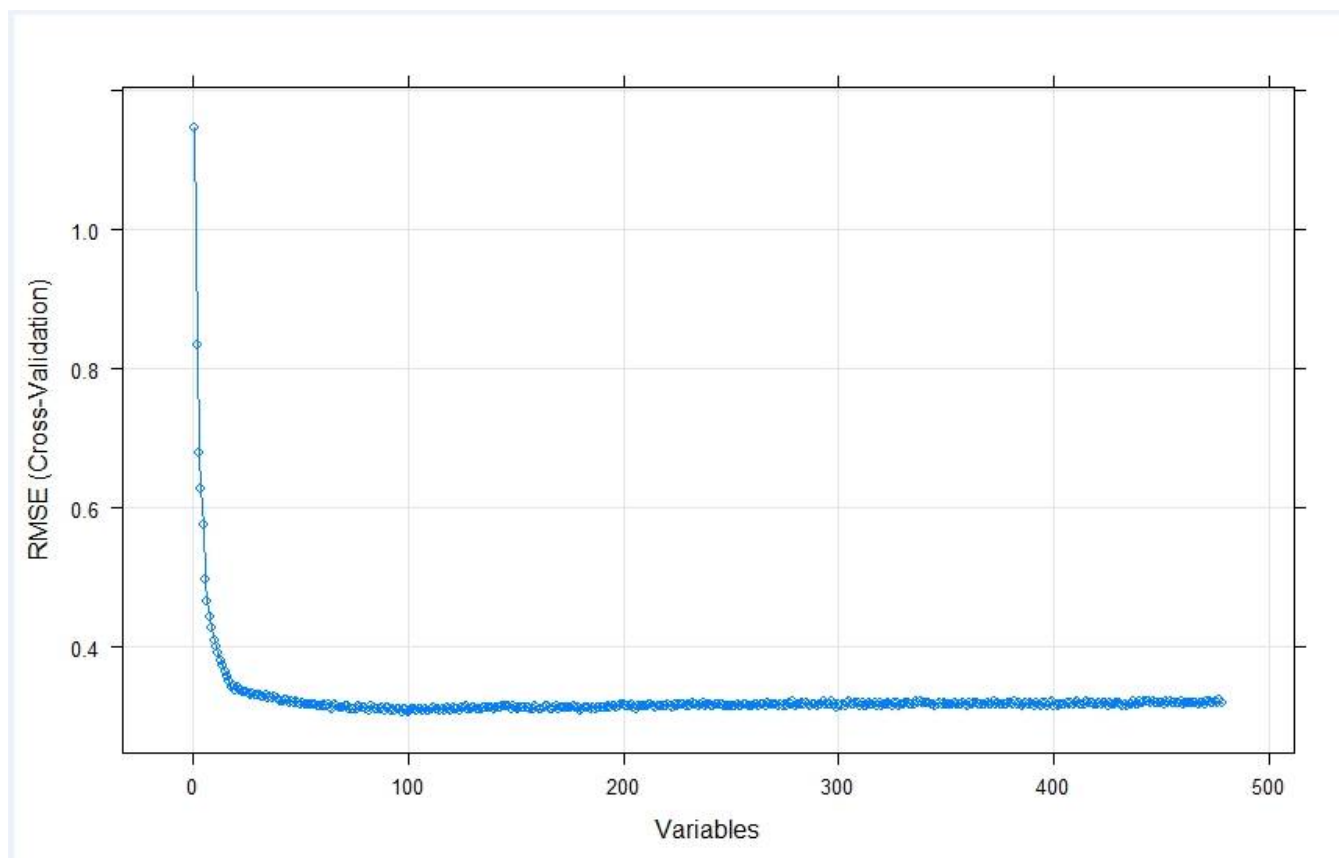
Figure 3. Importance of Variables Using Random Forest Recursive Feature Elimination Method.
