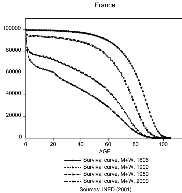
Figure 1: Period survival curves, men and women, France.
