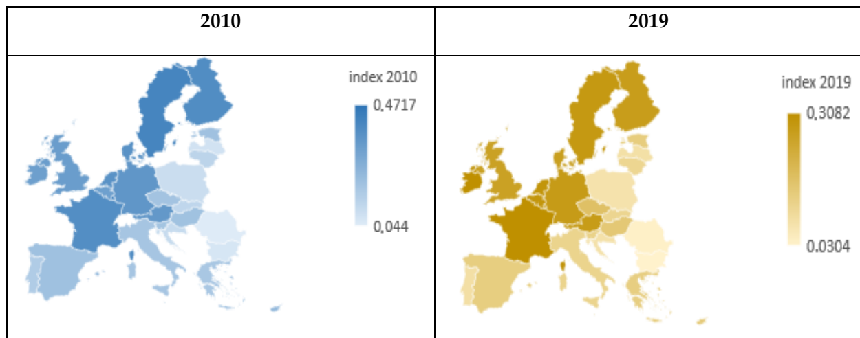
Figure 2. Comparison of the EU countries in terms of the value of the synthetic measure in 2010 and 2019. Source: Authors' own compilation based on Eurostat data; visualization supported by Bing, Geonames, Microsoft, TomTom.
