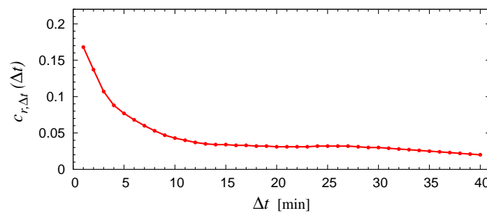
Figure A1. Empirical linear correlation function between two contiguous intervals of span \Delta t .
