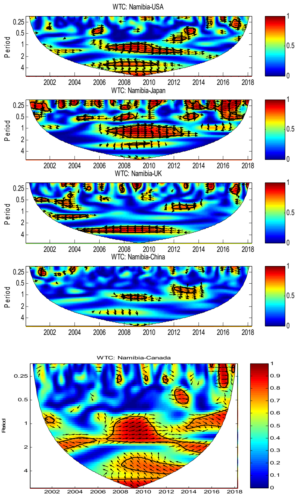
Figure 5. Pairwise wavelet coherence between selected nine African and five advanced countries.
