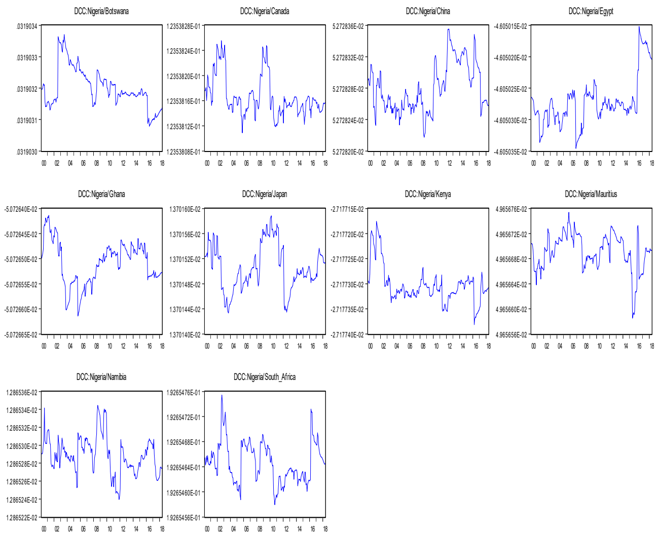
Figure 7. Dynamic conditional correlations plots between Nigeria and other countries. 5
