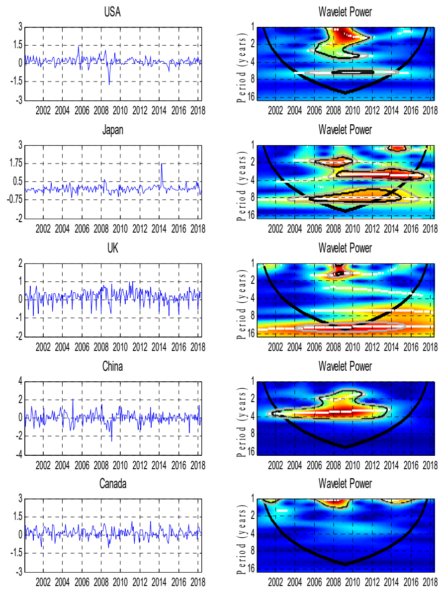
Figure 3. Wavelet power spectrum of inflation rates in selected five advanced countries.
