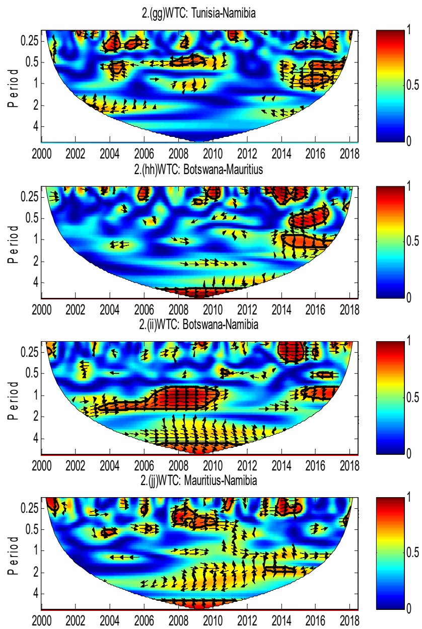
Figure 4. Pair wise wavelet coherence between selected nine African countries.
