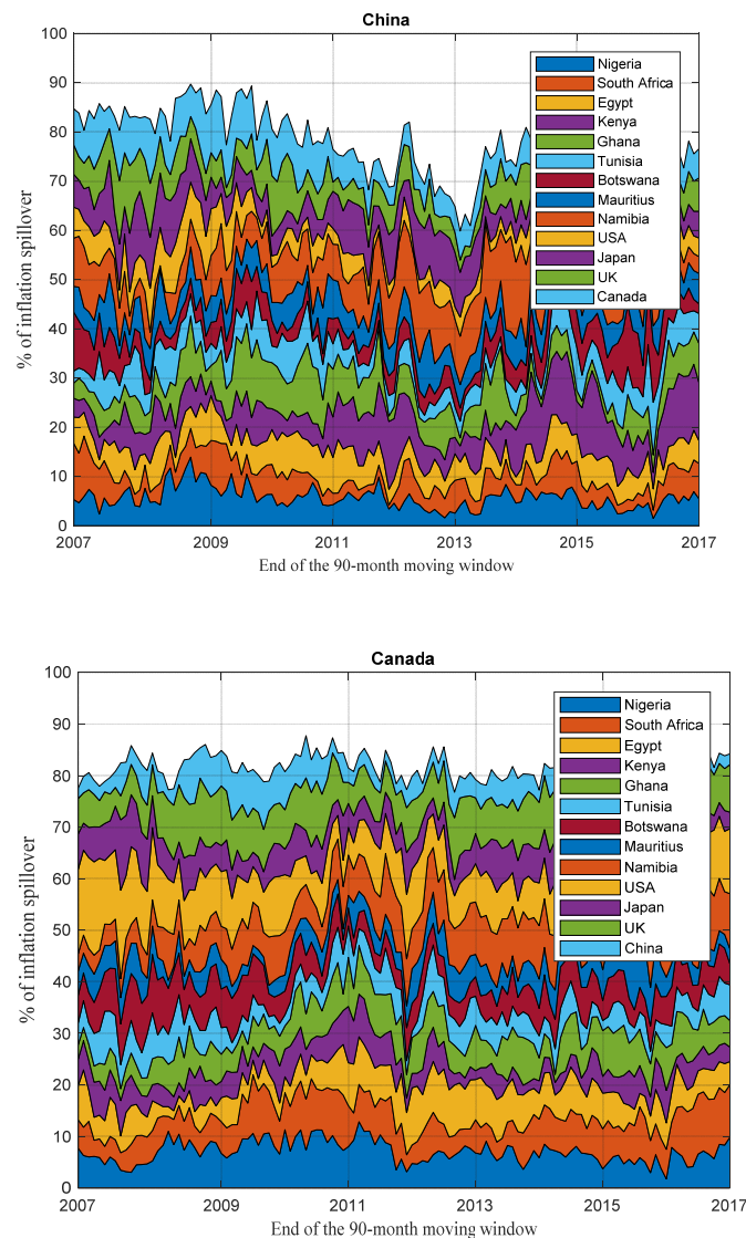
Figure 6. Inflation spill over across selected nine African and five advanced countries.
