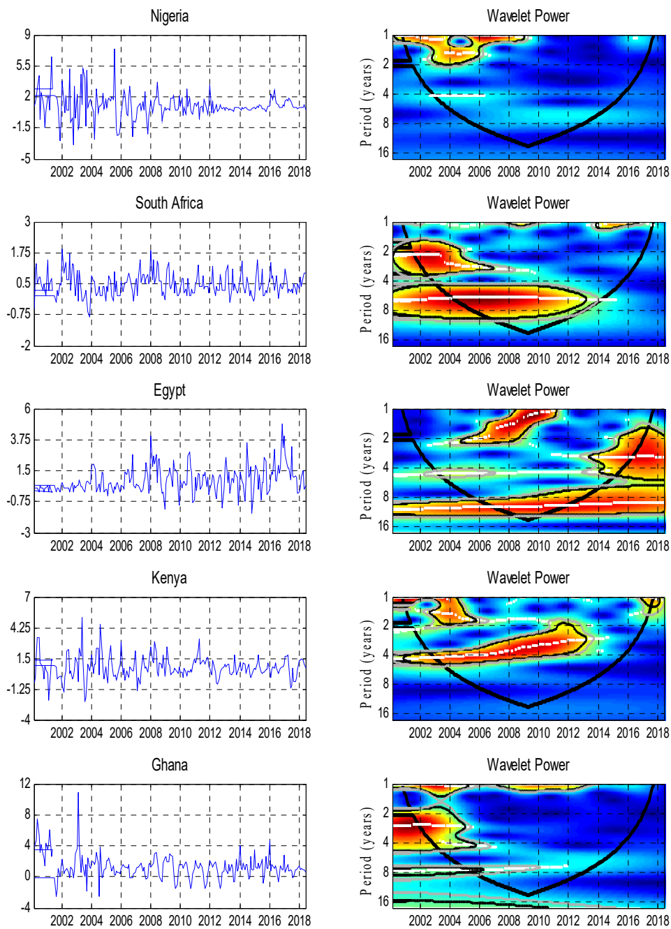
Figure 2. Wavelet power spectrum of inflation rates in selected nine African countries.
