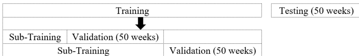
Figure 2. The 2-fold time-series cross-validation for weekly models.
