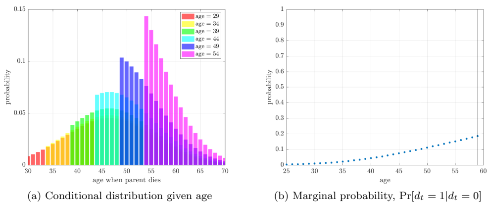
FIGURE C.1. INHERITANCE PROCESS
