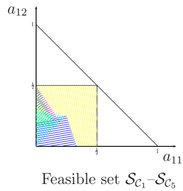
Figure 3: Feasible set \mathcal{S}_C .
