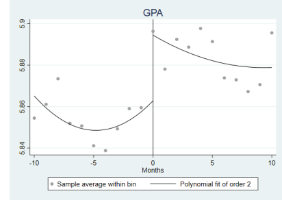
Figure 12: RD plot (grade point averages - p=2 )
