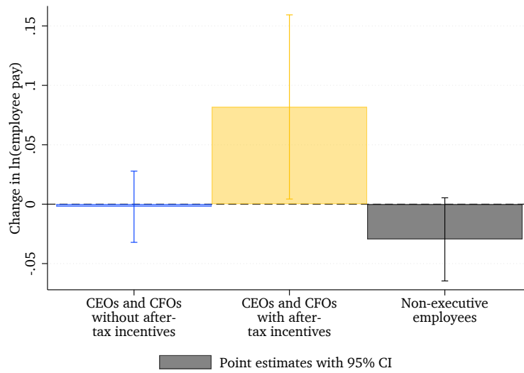
FIGURE 6 – Benchmark results
