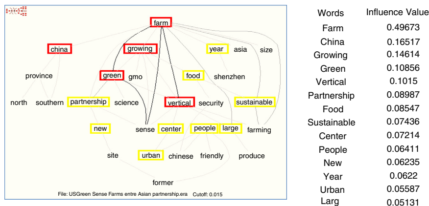
Fig. 1. Illustration of word network generated through CRA and important words. 1
