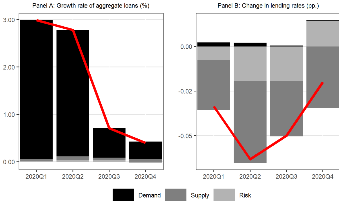
Figure 4: Decomposition
