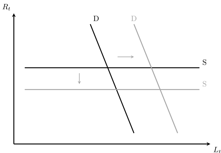
Figure 3: AD-AS diagram
