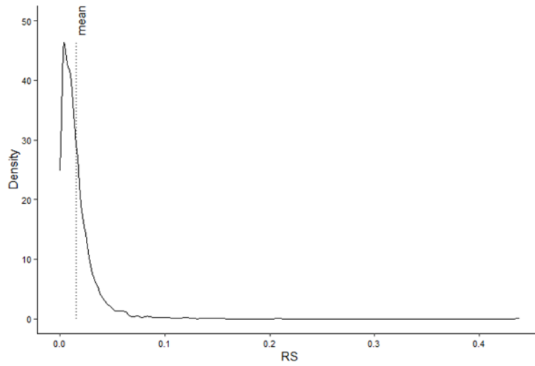
Figure 3. Density plot elucidating skewness for RS variable
