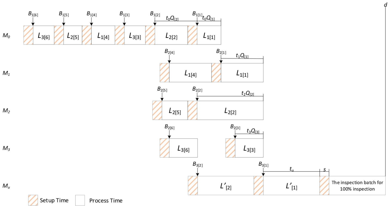
Figure 1. The Gantt Chart for Three-Stage-Flowshop with Job and Batch Processor
