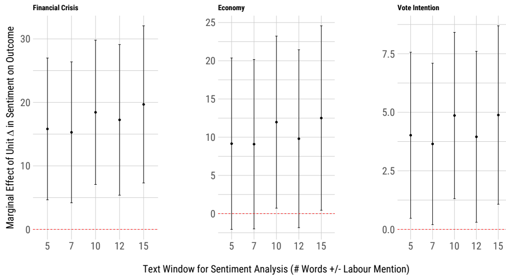
Figure B.2: Varying Text Window for Sentiment Score
