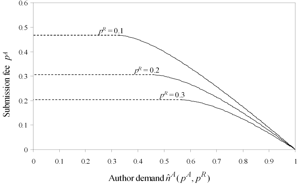
Figure 1: Discontinuities exhibited by reduced-form author demand in numerical example with uniformly-distributed benefits.
