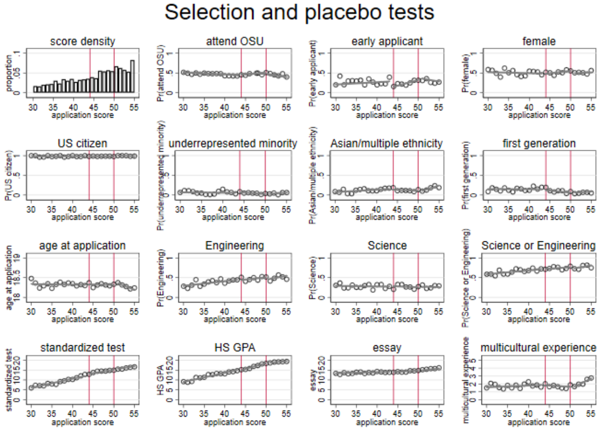
Figure 4: Selection and placebo tests
