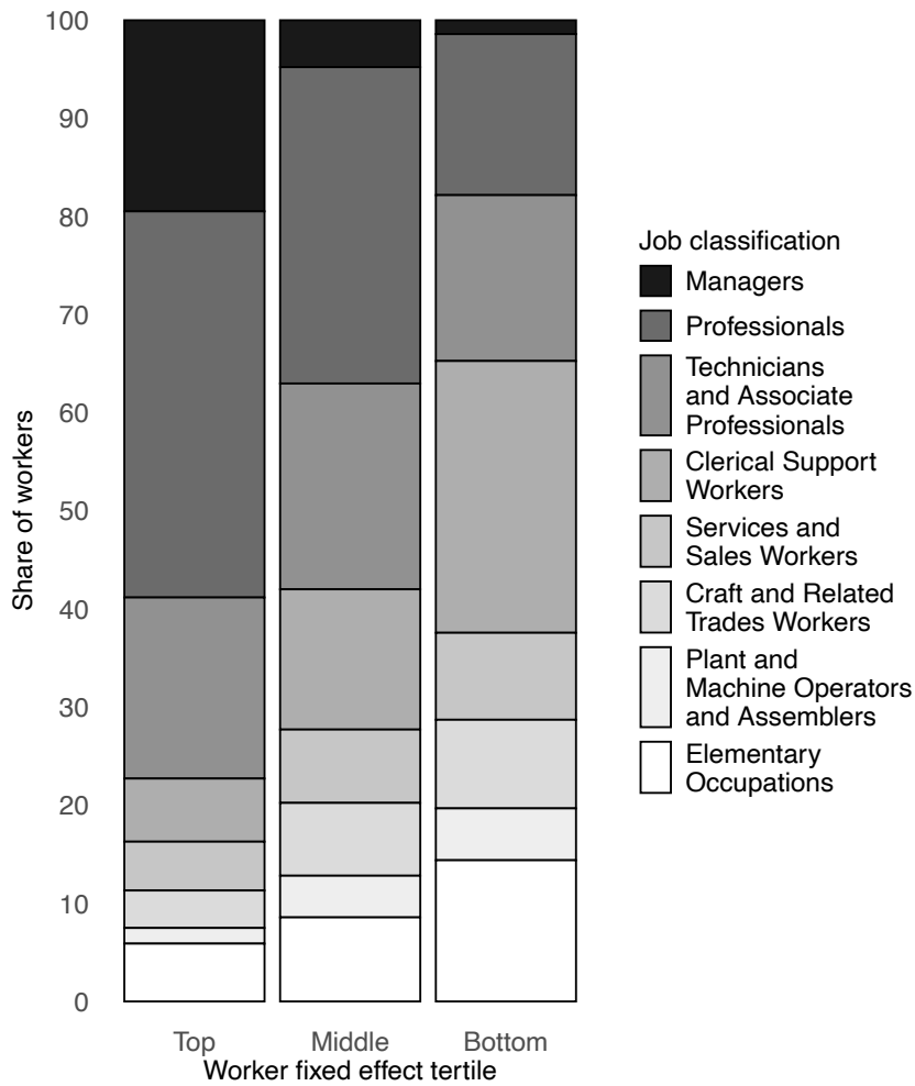
Figure 2: Occupations per worker fixed effect tertile.
