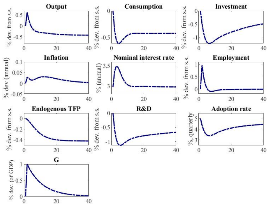
Figure 6: Impulse response to a one standard deviation government spending shock
