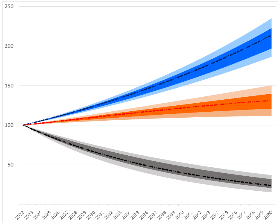
Fig. 3: Ambitious case. Per capita consumption (blue), population (orange), emissions (grey)
