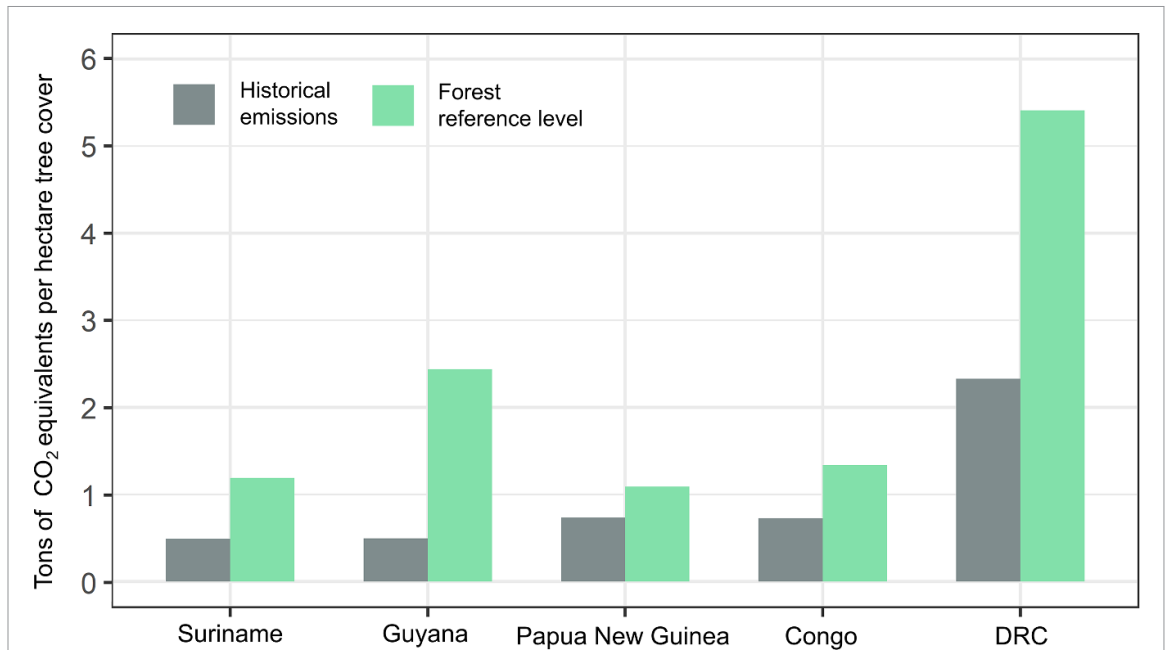
Figure 3. Mean historical emissions and proposed FRL. Future emissions were estimated from each country’s proposed FRL (in tons CO 2 per hectare). We used the tree cover data from Hansen et al (2013) as a baseline for the historical emissions. The historical emission periods range from 10 to 14 years between 2000 and 2015 (depending on the country’s FRL).
