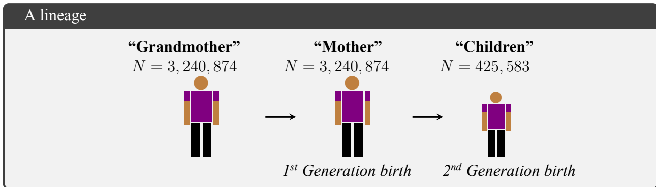
Figure 2: Schematic Representation of a Lineage
