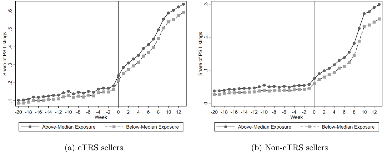
Figure 2: Parallel trends
