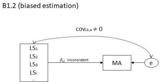
Figure 3: Endogeneity in multivariate models
