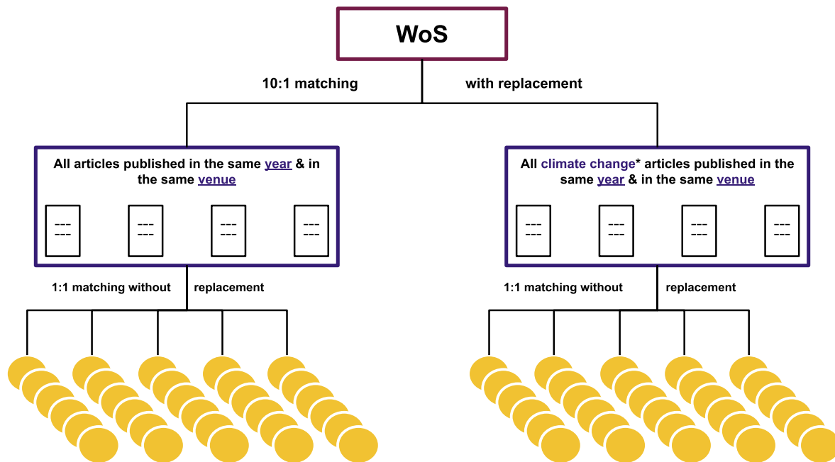
Figure S2: Matching scheme. A schematic representation of the matching procedure used in the empirical analysis. The right end side refer to the construction of the baseline control group; while the left end side refers to the climate control.
