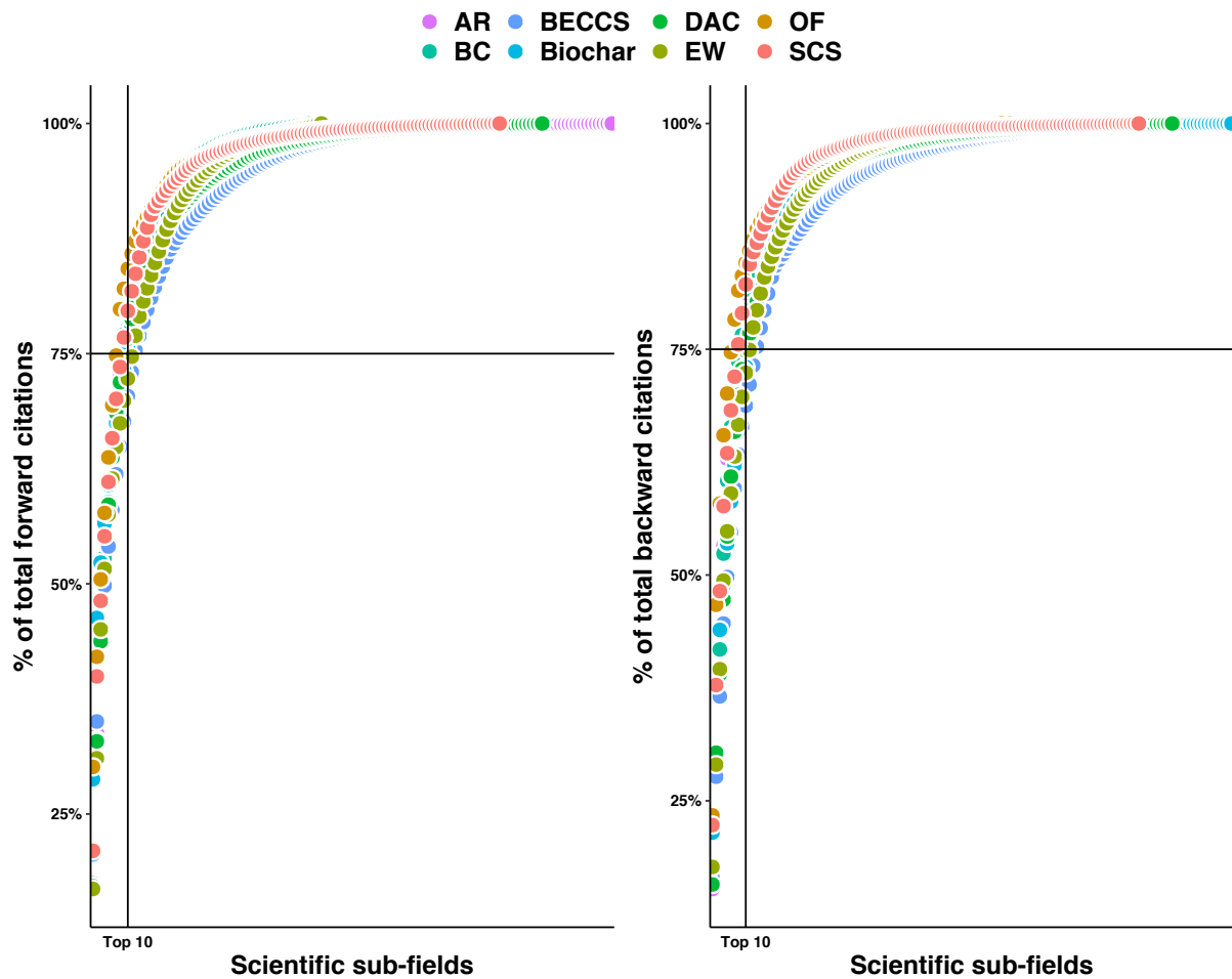
Figure S6: Pareto plot. Cumulative percentage of the total number of forward and backward scientific citations by NETs. The horizontal reference line marks the 75% of total citations. The vertical reference line indicates the 10 largest scientific sub-fields.
