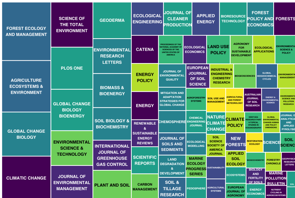
Figure S3: Top NETs Venues. Treemap listing the most representative venues for NETs articles. The map include academic journals that published at least 10 paper related to NETs.
