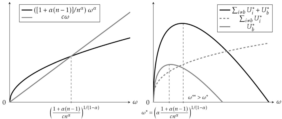
Fig. 6. Net payoffs possibilities in the Nash equilibrium in the water bank example.
