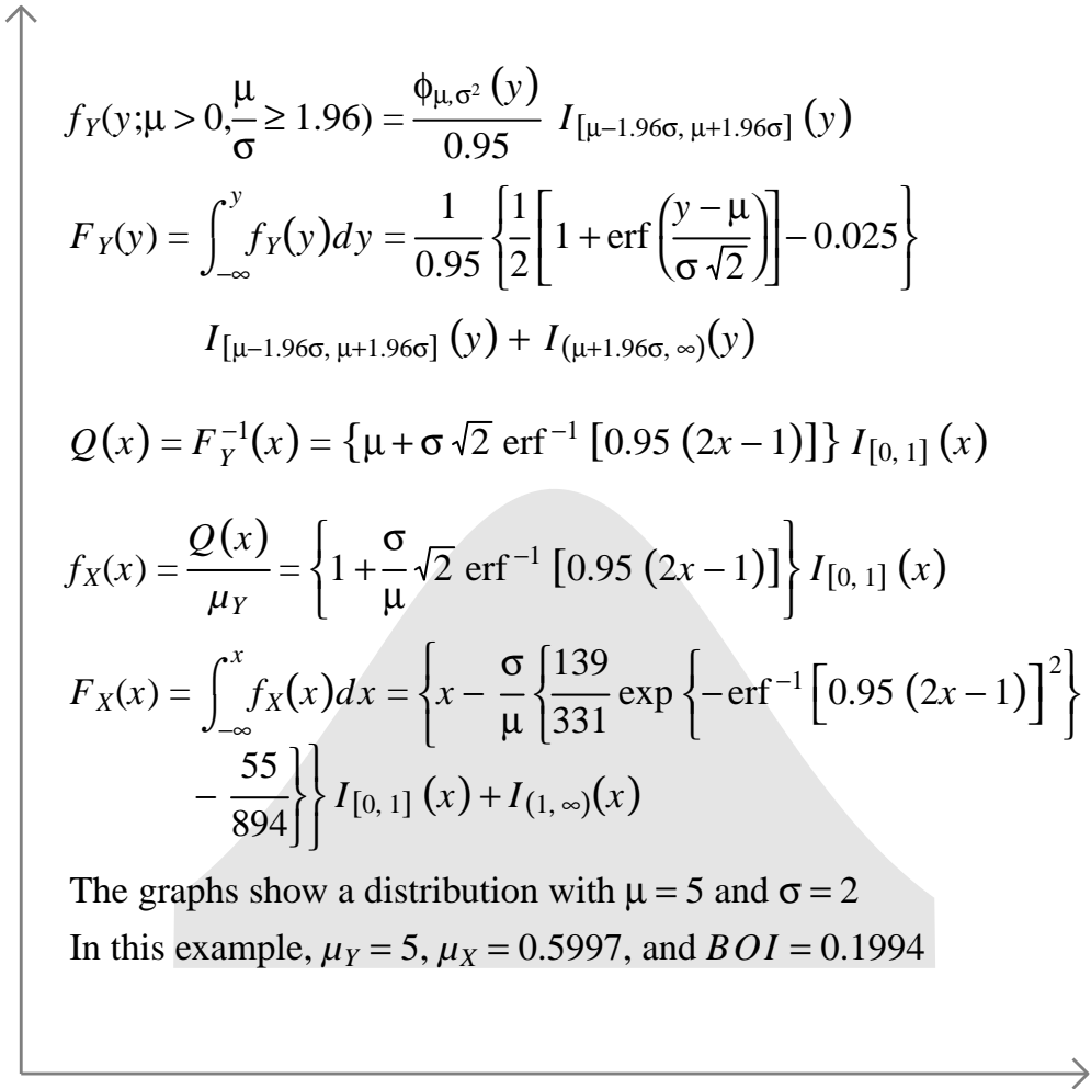
Figure A3.14 – Normal distribution symmetrically truncated 95% 1. Probability density function of Y, f_Y(y)
