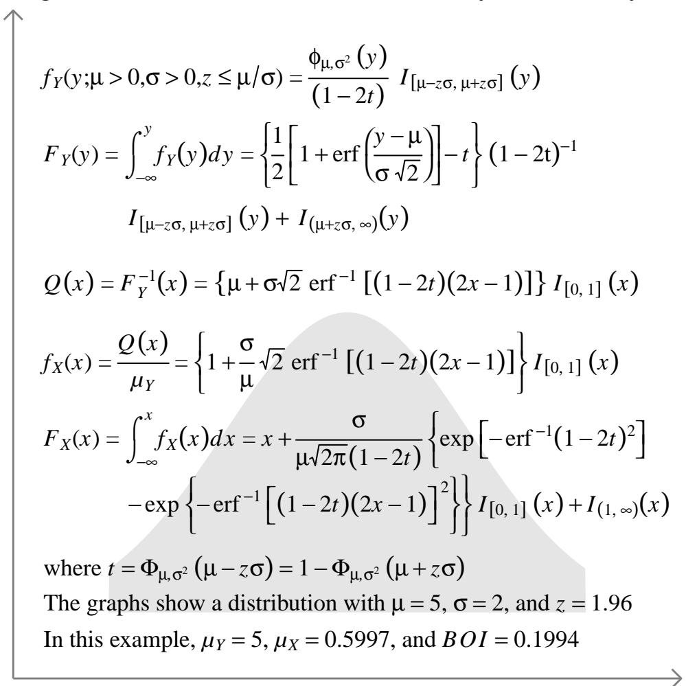
Figure A3.13 – Normal distribution symmetrically truncated
