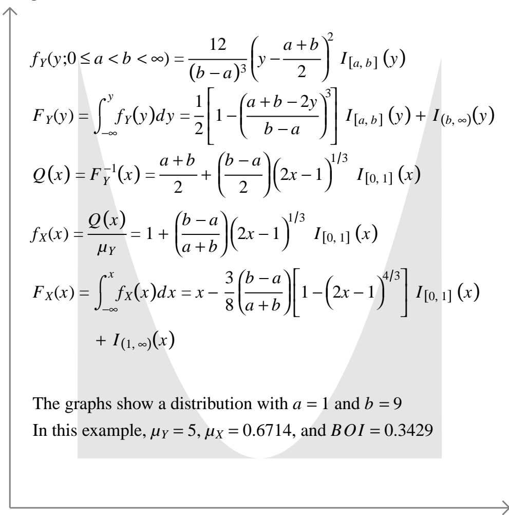
Figure A3.28 – U–Quadratic distribution
