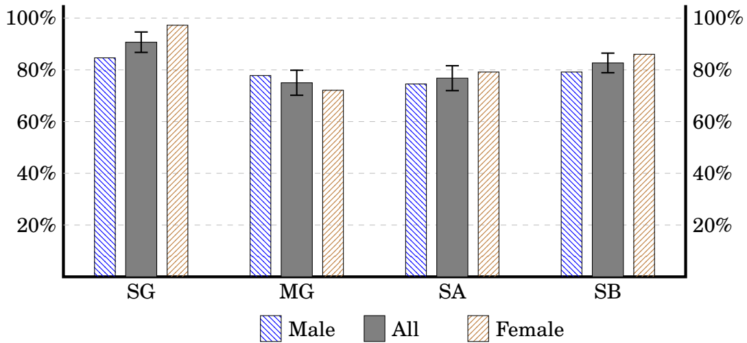
Figure 3: Proportions of allocating downward, by gender composition SG/MG=rank r - 1 and r + 1 have the same/different gender. SA/SB=the rank above/below has same gender.
