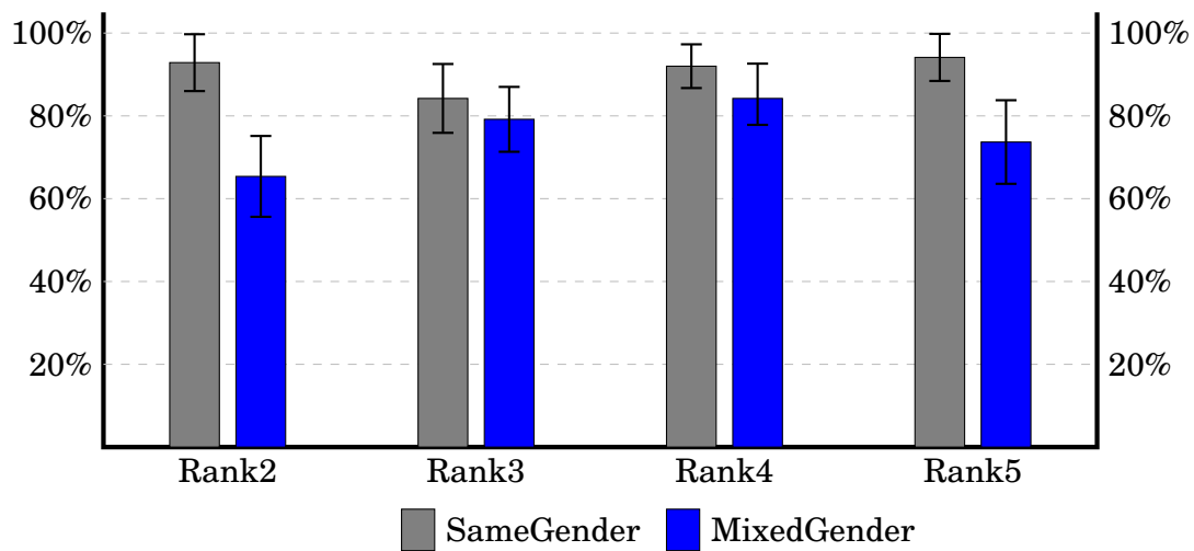
Figure 4: Proportions of decisions allocating to the Rank-Below in the SG and MG, by rank
