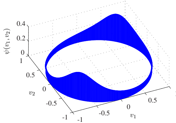
Figure 7: Spectral density of a 2-dimensional unit random vector generated by \Sigma_{11} = \Sigma_{22} = 1 and \Sigma_{12} = \Sigma_{21} = 0.7 .
