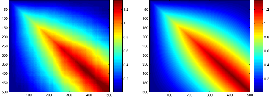
Figure 8: Spectral estimator for multivariate t -distributed data ( n = 1000, d = 500 ) with three degrees of freedom (left) and the corresponding true dispersion matrix (right).
