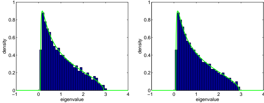
Figure 9: Eigenspectra obtained by the spectral estimator for univariate (left) and multivariate (right) uncorrelated t -distributed data ( n = 1000, d = 500 ) with five degrees of freedom.
