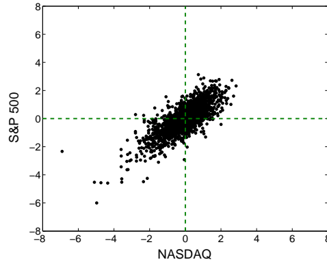
Figure 2: NASDAQ vs. S&P 500 GARCH(1,1) residuals from 1993-01-01 to 2000-06-30 ( n = 1892 ).
