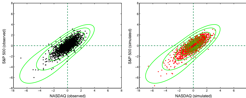
Figure 4: Observed GARCH(1,1) residuals of NASDAQ and S&P 500 (left hand) and simulated generalized elliptically distributed residuals ( n = 1892 ) (right hand).
