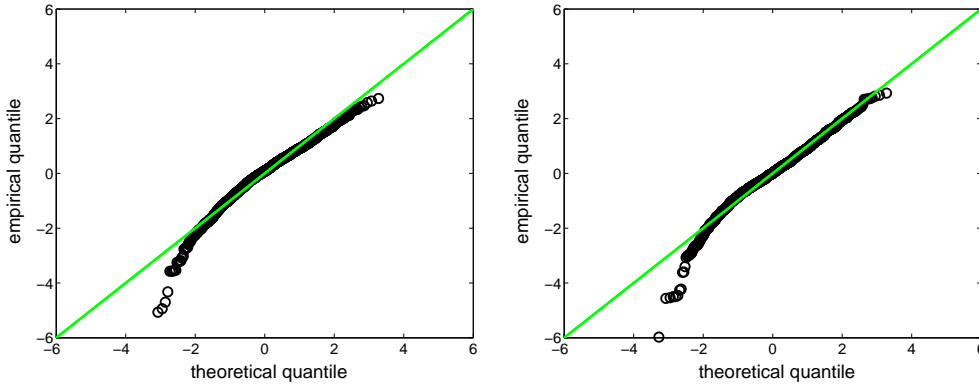
Figure 1: Normal QQ-plots of GARCH(1,1) residuals of daily log-returns of NASDAQ (left hand) and S&P 500 (right hand) from 1993-01-01 to 2000-06-30 ( n = 1892 ).
