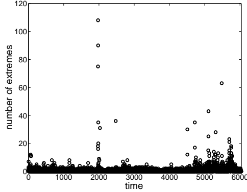
Figure 3: Number of extremes in the S&P 500 during 1980-01-02 to 2003-11-26.
