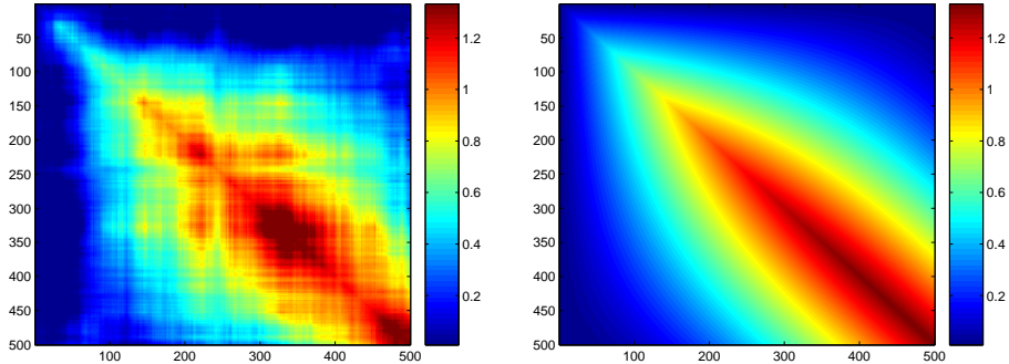
Figure 6: Normalized sample covariance matrix for multivariate t -distributed data ( n = 1000, d = 500 ) with three degrees of freedom (left) and the corresponding true dispersion matrix (right).
