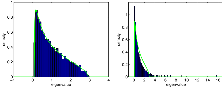
Figure 5: Eigenspectra obtained by the sample covariance matrix of univariate (left) and multivariate (right) uncorrelated t -distributed data ( n = 1000, d = 500 ) with five degrees of freedom.
