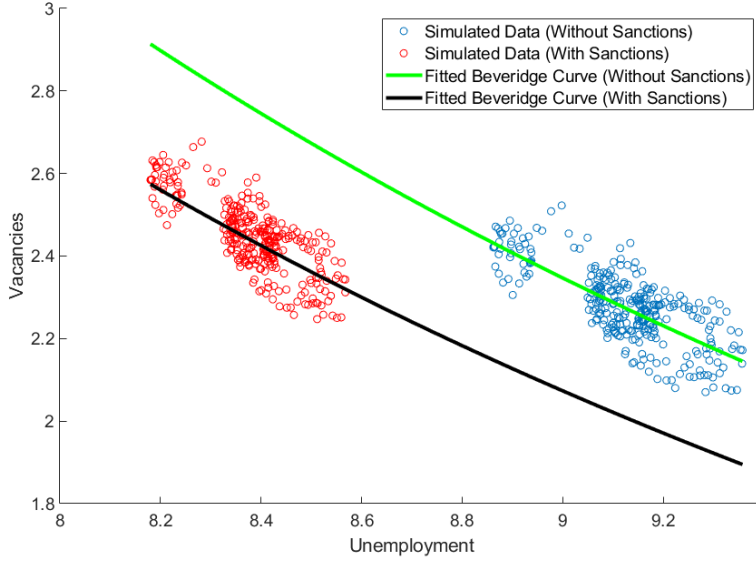
Figure 5: Beveridge Curve
