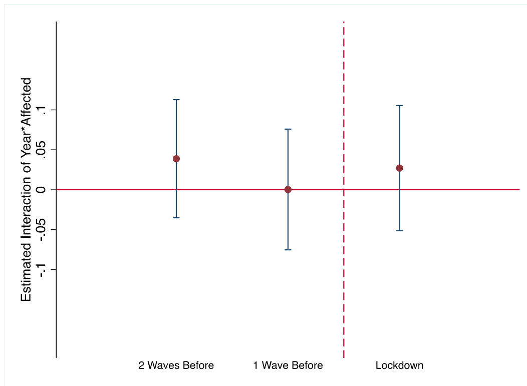
Figure 4. Event study
