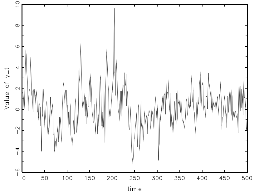
Figure 2. Sample path for DGP1-1 with \gamma_1 = 0.3 .
