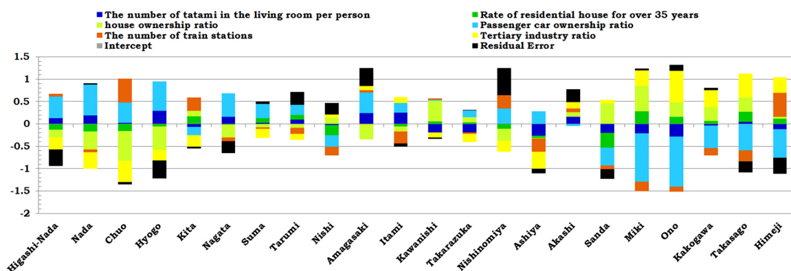
Fig. 6. Approach 2 / stepwise estimation WLS-2. Estimation results of residual errors and urban amenities.
