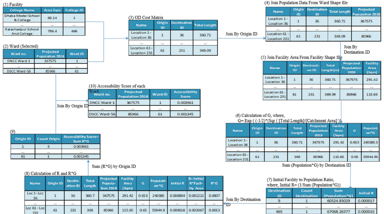
Fig. 3. Work flow for calculating supply-to-demand ratio and spatial accessibility (Step 1 and 2) (Source: Author, 2018).
