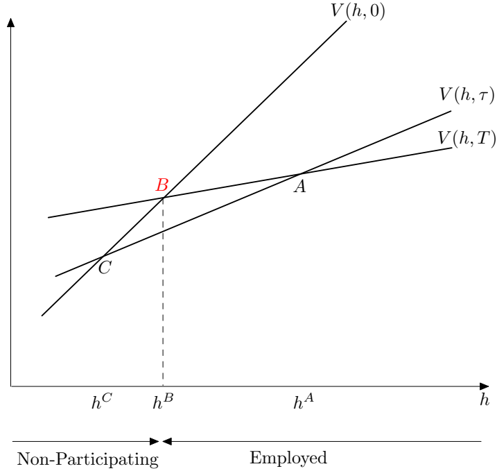
Figure 3: Career Diagram without Unemployment
