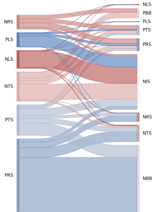
(b) Sankey plot showing consecutive events where the initial events include only events identified as shocks.
