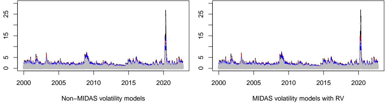
Figure 4: Total volatility components \sigma_t .
