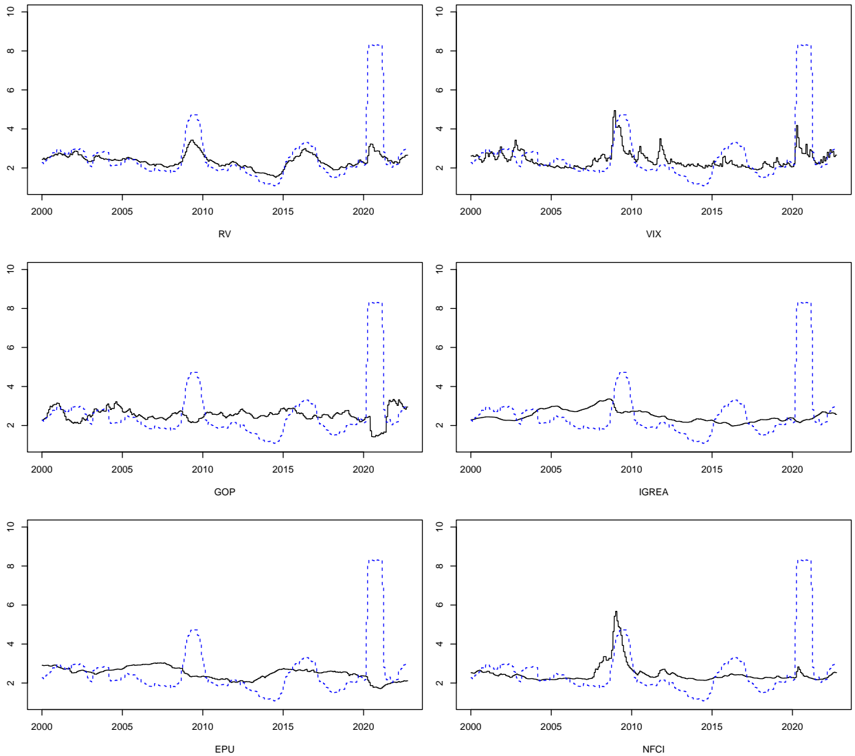
Figure 3: Long-term volatility components \sqrt{\kappa_\tau} obtained from the GAS-MIDAS models with t -innovations and leverage effect.
