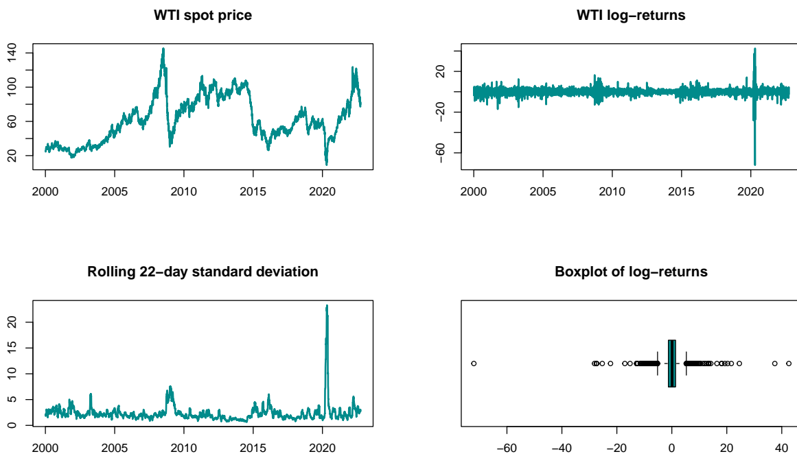
Figure 1: Crude oil spot prices, de-meaned log returns, rolling 22-day standard deviation (right-aligned), and a boxplot for the de-meaned log returns from January 4, 2000 to September 30, 2022.
