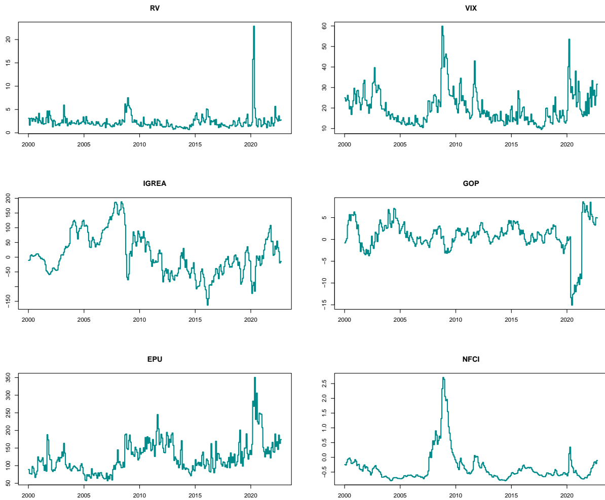
Figure 2: Plots for the macroeconomic variables from January 4, 2000 to September 30, 2022.
