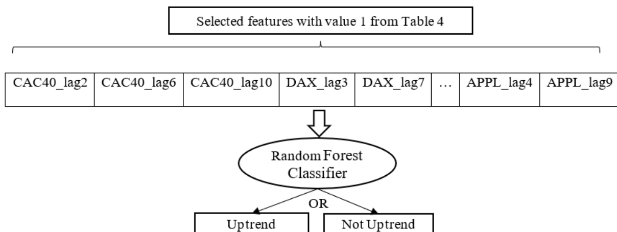
Figure 4. Random forest classifier.
