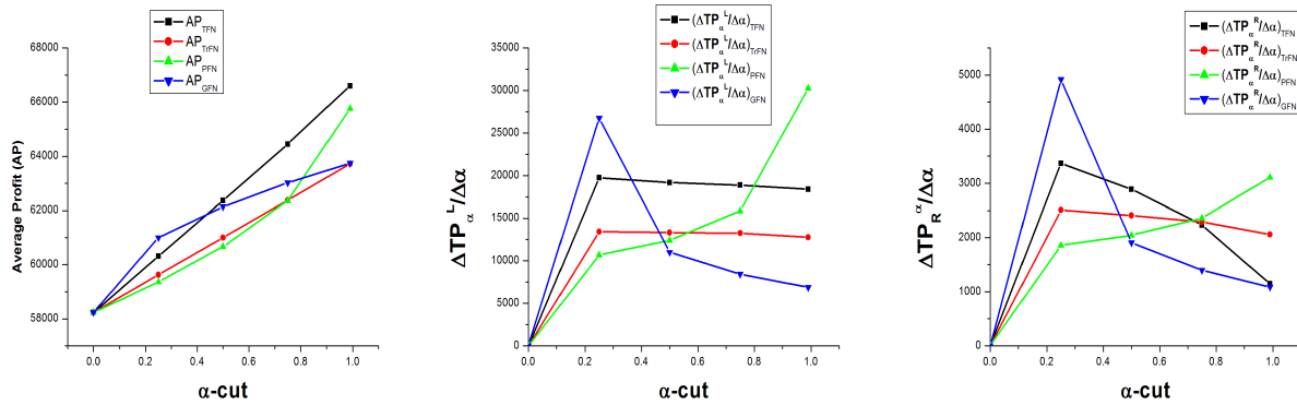
Figure 2. Graphical representation of average profit with \alpha .
