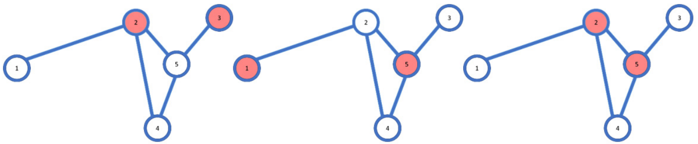
Figure 1. A five node network with three possible Dominating Sets.
