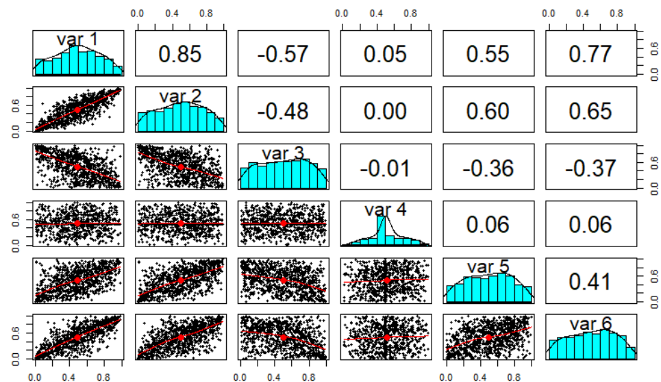
Figure 5. Scatterplots between pseudo-observations of each pair of indexes in the lower triangular panels, histograms of each marginal in the diagonal, and Pearson’s correlation coefficients in the upper triangular panels.
