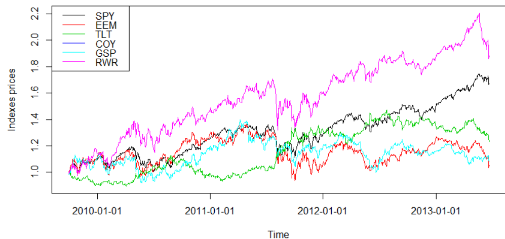
Figure 1. Performance of price movements of each index over the historical record.
