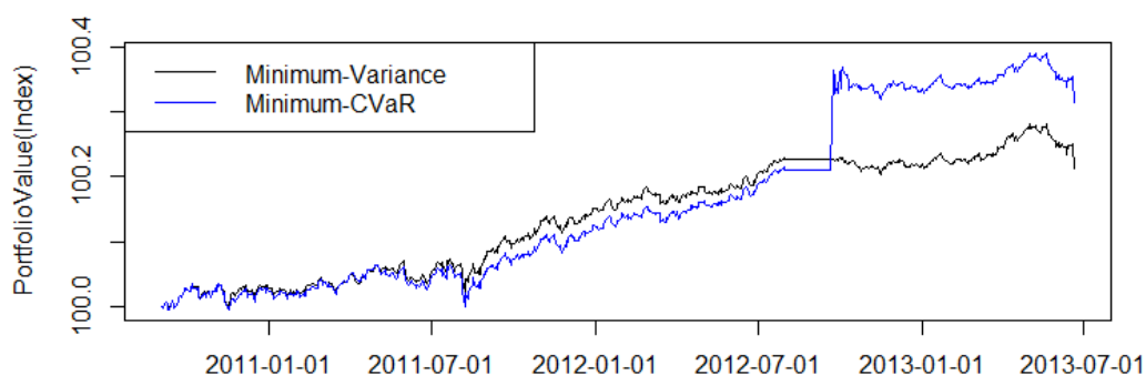
Figure 6. Trajectory of WCVaR and minimum-variance portfolio values.
