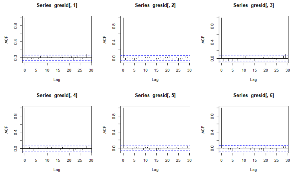
Figure 4. Plots of autocorrelation functions (ACF).
