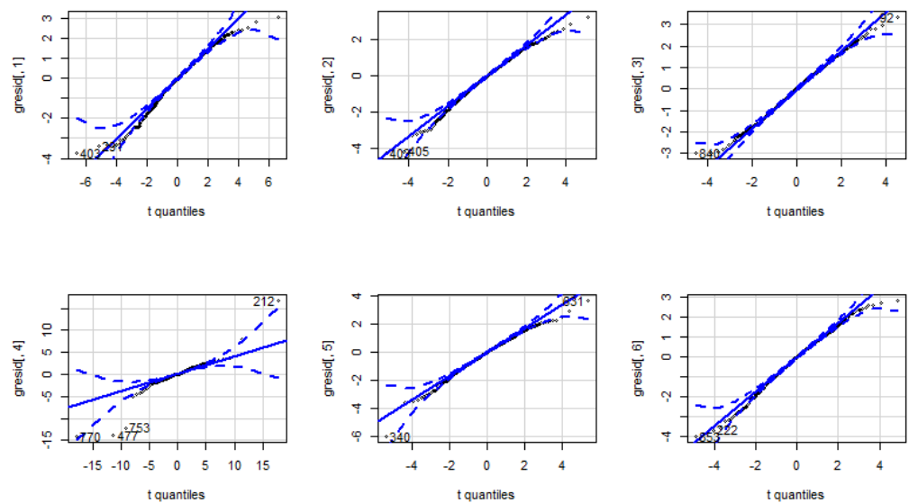
Figure 3. The Student's t-quantile functions of the residuals of GARCH(1,1) for each marginal.
