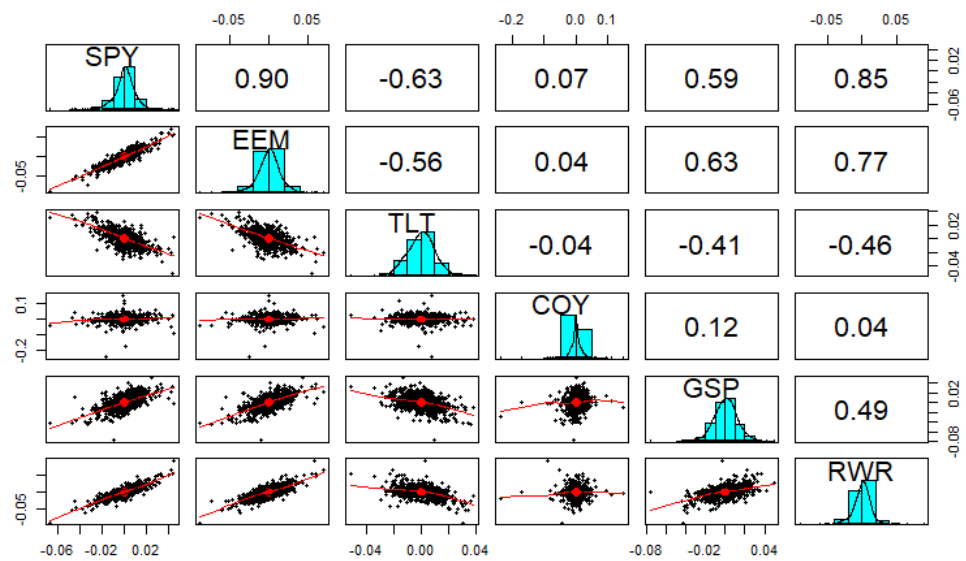
Figure 2. Scatterplots between each pair of index returns in the lower triangular panels, histograms of each marginal in the diagonal, and Pearson's correlation coefficients in the upper triangular panels.
