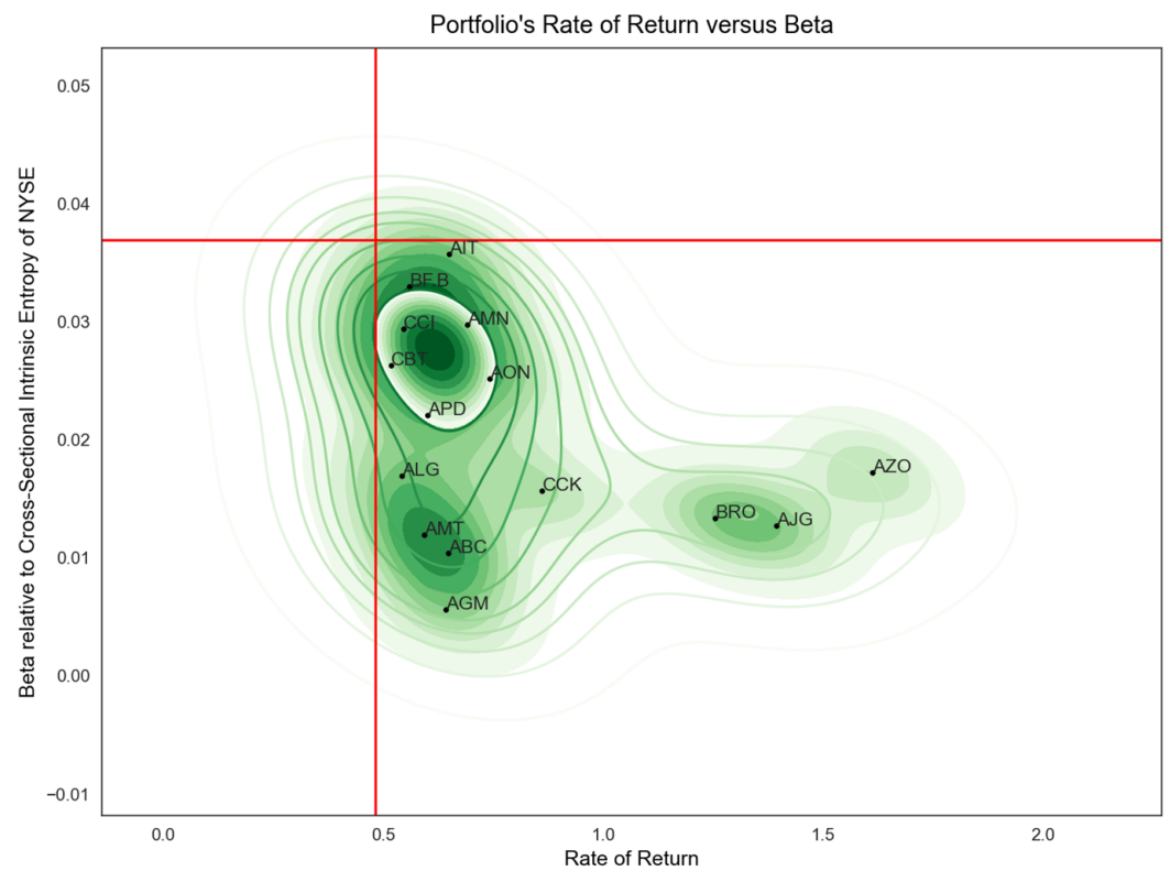
Figure 3. A set of 15 NYSE symbols that outperformed the S&P500 index in terms of rate of return without being exposed to higher risk (950-day trading interval, from 2 April 2018 to 26 August 2022).
