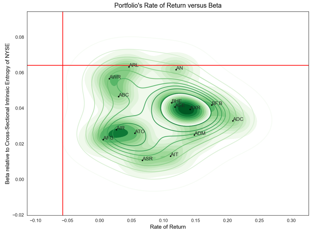
Figure 1. A set of 15 NYSE symbols that outperformed the S&P500 index in terms of rate of return without being exposed to higher risk (125-day trading interval, from 1 March 2022 to 26 August 2022).
