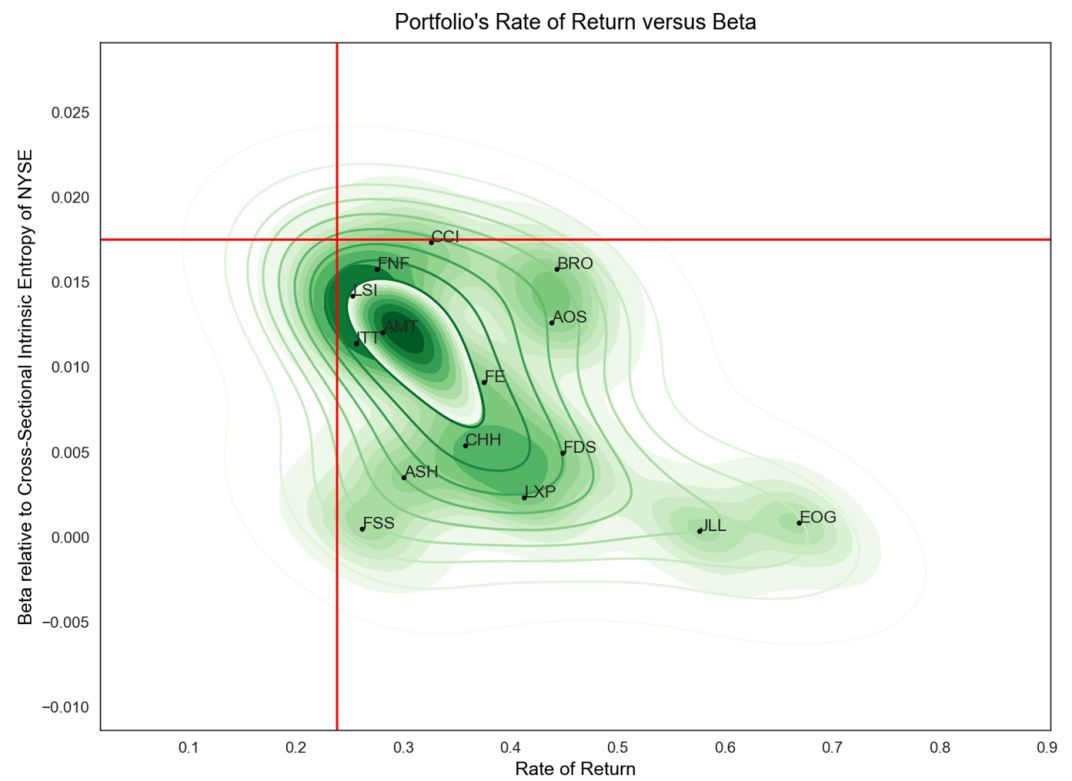
Figure 2. A set of 15 NYSE symbols that outperformed the S&P500 index in terms of rate of return without being exposed to higher risk (250-day trading interval, from 5 October 2020 to 20 December 2021).
