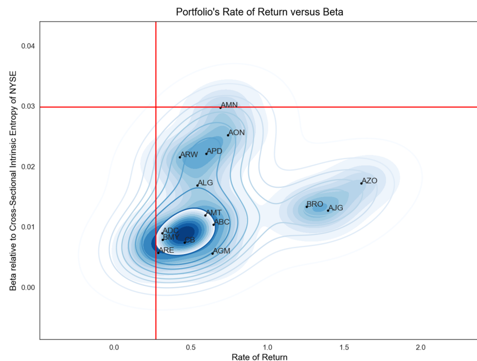
Figure A3. A set of 15 NYSE symbols that outperformed the DJIA index in terms of rate-of-return without being exposed to higher risk (950-day trading interval, from 2 April 2018 to 26 August 2022).
