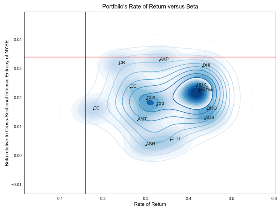
Figure A2. A set of 15 NYSE symbols that outperformed the DJIA index in terms of rate-of-return without being exposed to higher risk (250-day trading interval, from 5 October 2020 to 20 December 2021).
