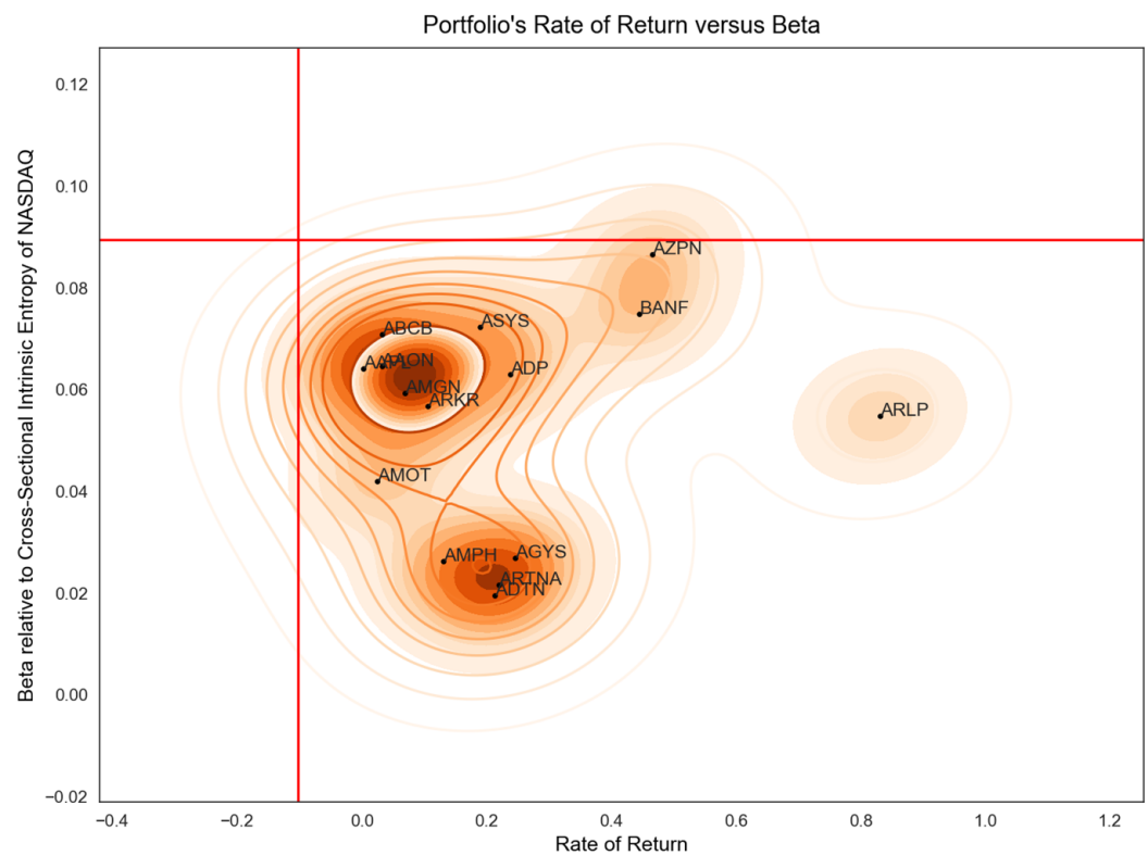
Figure 4. A set of 15 NASDAQ symbols that outperformed the NASDAQ Composite index in terms of rate of return without being exposed to higher risk (125-day trading interval, from 1 March 2022 to 26 August 2022).
