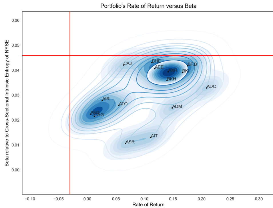
Figure A1. A set of 15 NYSE symbols that outperformed the DJIA index in terms of rate of return without being exposed to higher risk (125-day trading interval, from 1 March 2022 to 26 August 2022).
