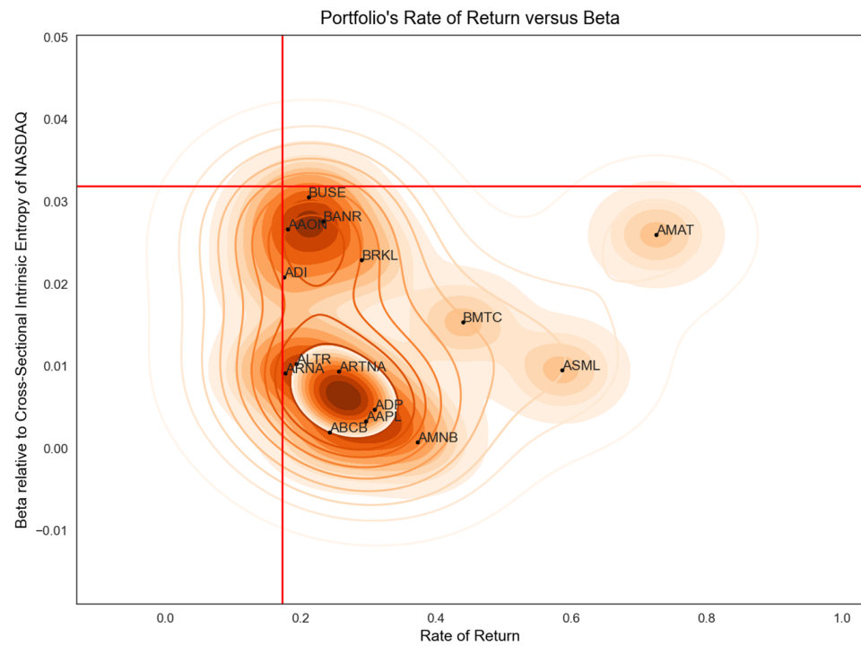
Figure 5. A set of 15 NASDAQ symbols that outperformed the NASDAQ Composite index in terms of rate of return without being exposed to higher risk (250-day trading interval, from 5 October 2020 to 20 December 2021).
