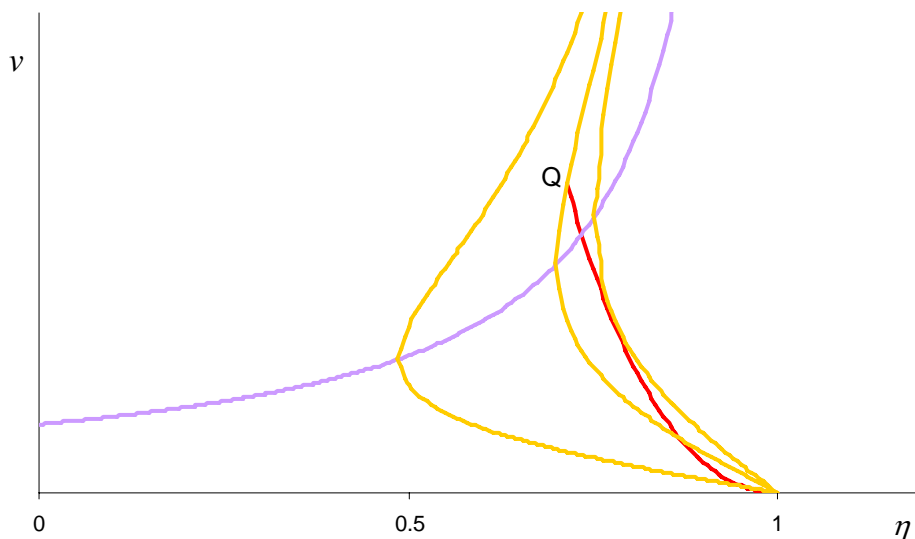
Figure 6: Origin of the Efficient Locus Q above the Bifurcation Locus
