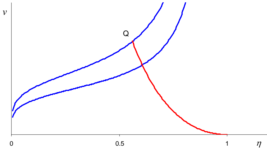
Figure 4: Equation (56) (blue) with Increasing N
