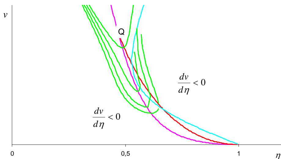
Figure 11: Physical per capita consumption with an “intermediate” value of \lambda
