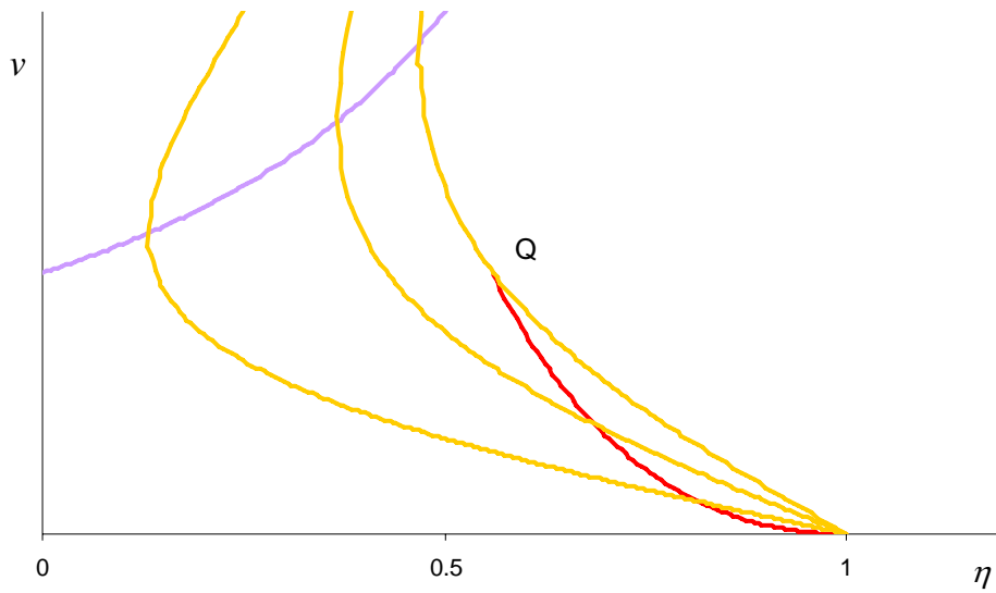
Figure 5: Bifurcation Locus (violet) and Different Levels of Physical Capital (gold)
