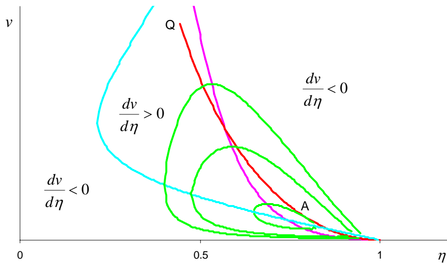
Figure 10: Physical Per Capita Consumption with a “Small” \lambda
