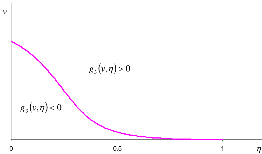
Figure 7: The g_3(v, \eta) = 0 Locus (pink)
