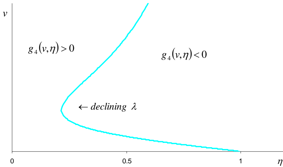
Figure 8: The g_4(v, \eta) = 0 Locus (cyan)
