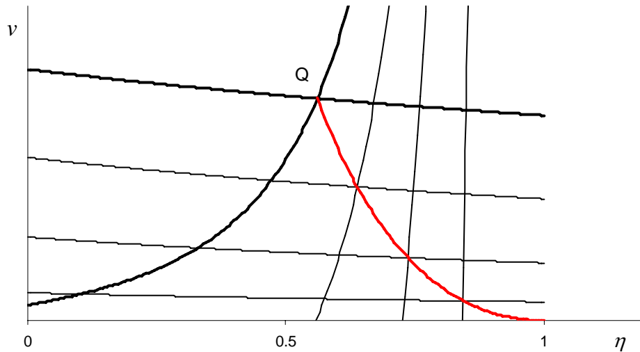
Figure 3: The Locus of Efficient Points (red) if Inequality (46) Holds
