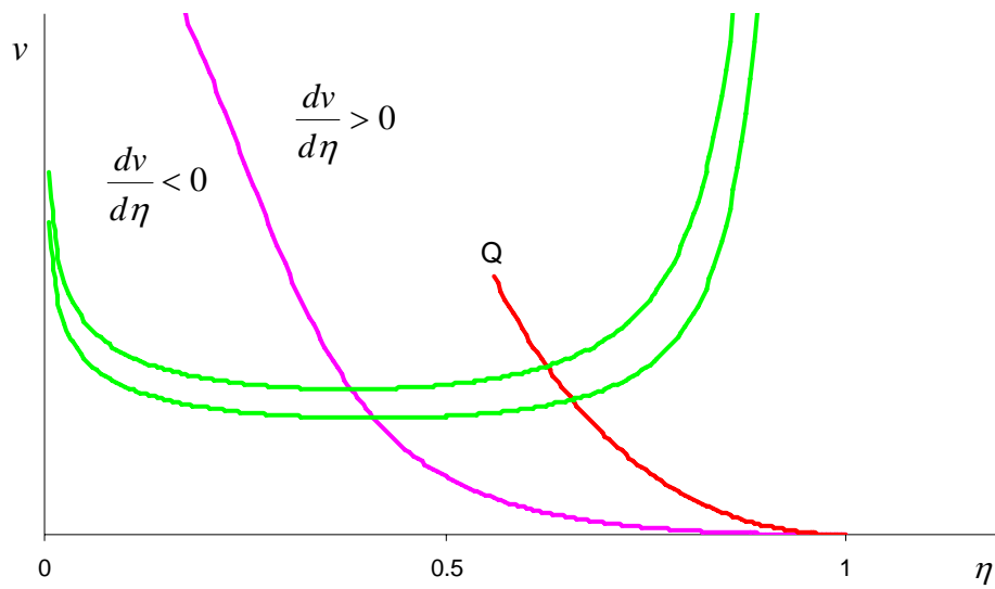
Figure 9: Physical Per Capita Consumption with a “Large” \lambda
