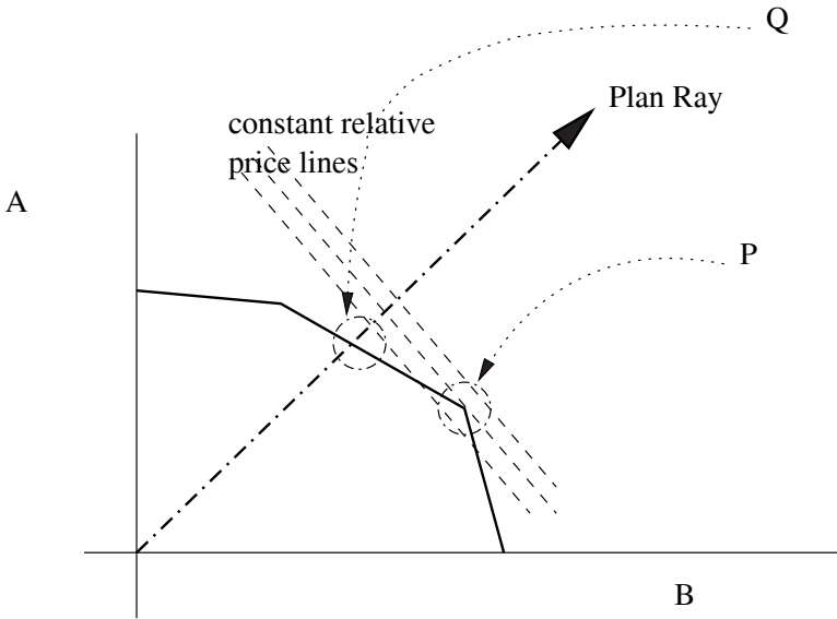
Figure 2: Comparison of the Western and Soviet versions of linear programming
