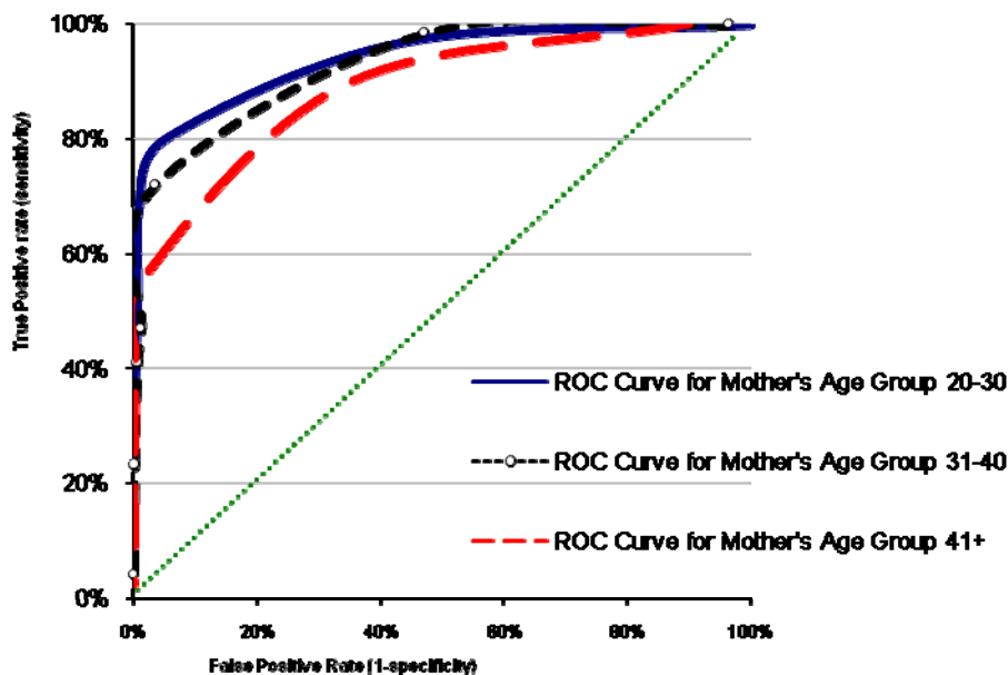
Figure 1: The ROC Curve
