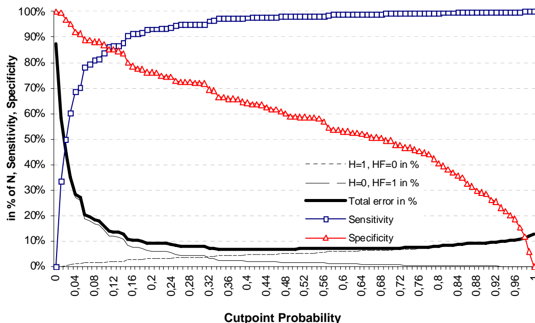
Figure 2: The Optimal Cutoff Value
