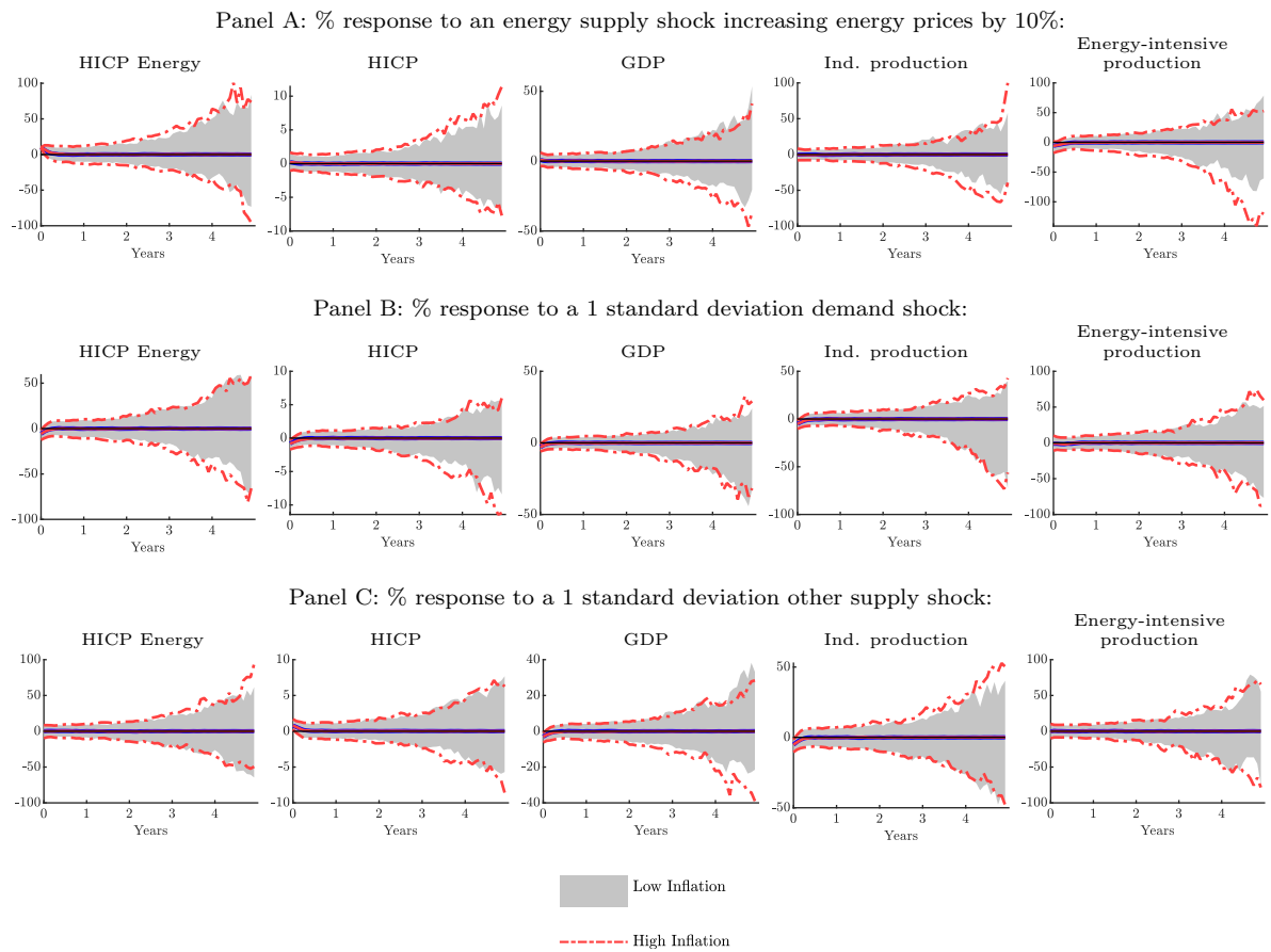
Figure 14: Nonlinear Impulse Response Priors
