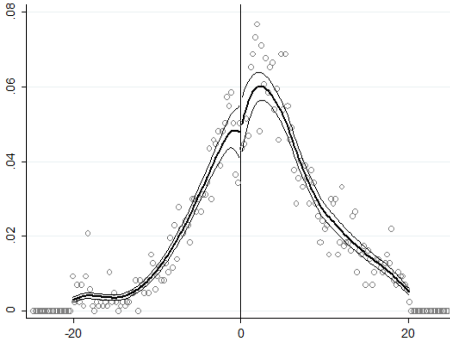
Figure 1: Manipulation of the forcing variable at the cut-off
