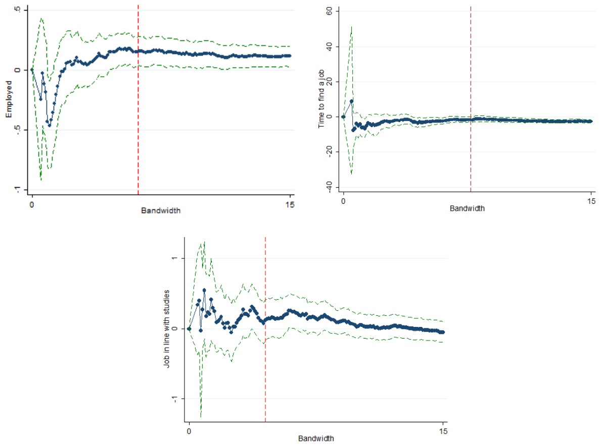
Figure 5: Sensitivity to different bandwidths – Fuzzy RDD
