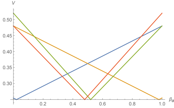
Figure 9: Value functions: blue v\left((1, \frac{1}{2} + \delta), \beta_a\right) , yellow v\left((\frac{1}{2} + \delta', 1), \beta_a\right) , orange v\left((1, 0), \beta_a\right) , green v\left((0, 1), \beta_a\right) .
