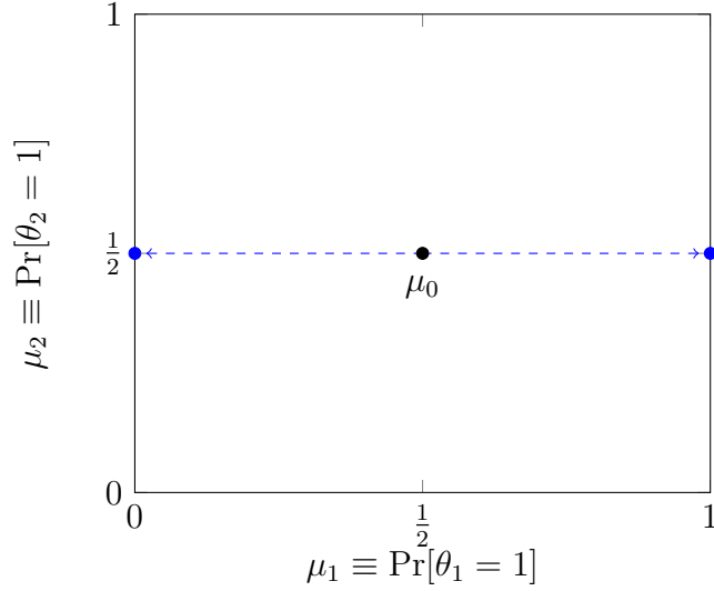
Figure 3: The blue dots represent the posteriors from the policy that secures v\left((1, \frac{1}{2}), \hat{F}_a\right) .
