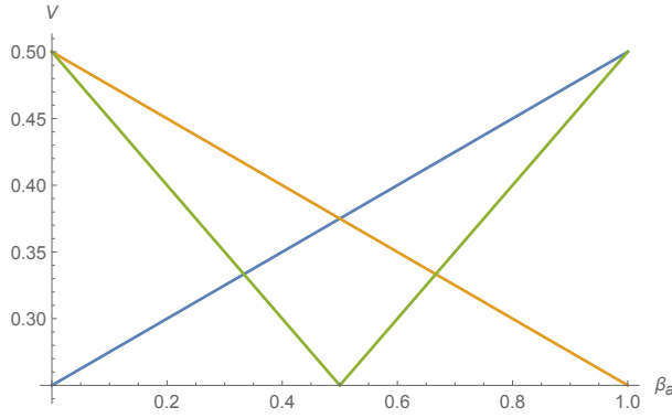
Figure 6: Value functions: blue v((1, \frac{1}{2}), \beta_a) , orange v((\frac{1}{2}, 1), \beta_a) , green v((1, 0), \beta_a) .
