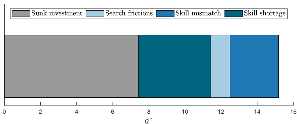
Figure 7: A schematic representation of the decomposition of the scrapping age of technologies in the presence of aggregate skill shortage.
