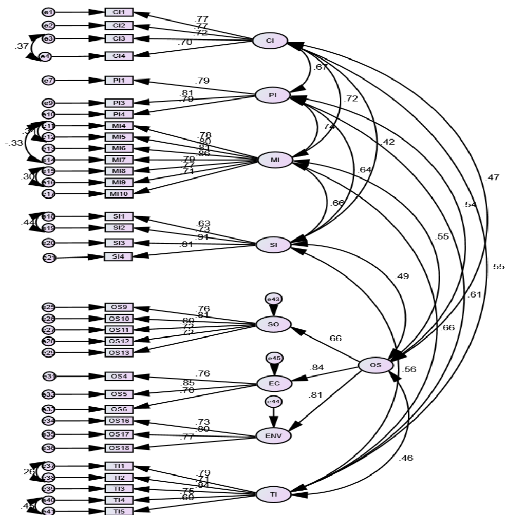
Figure 2: Measurement model
