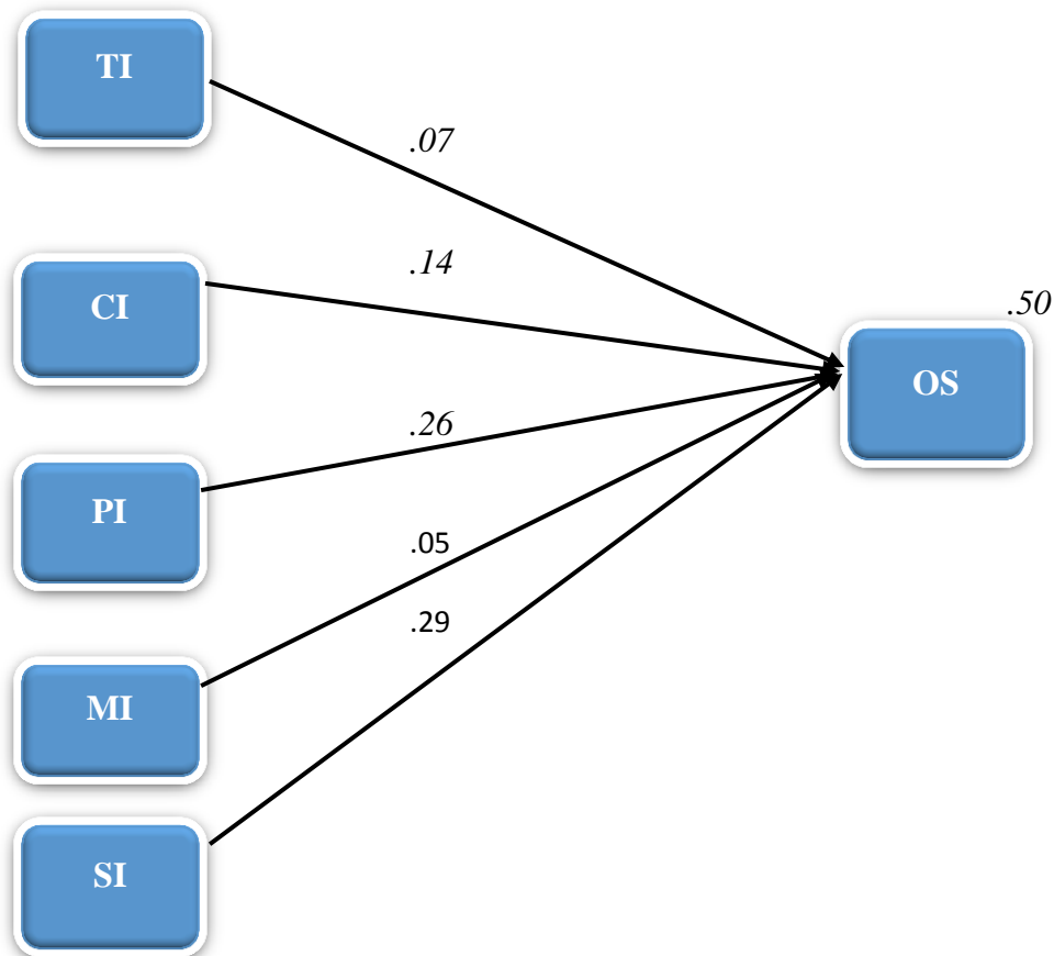
Figure 3: Structural Model
